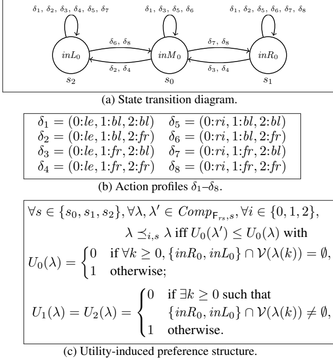
Figure 2: CGMRP M_{rs} for the robots' scenario: (a) state transitions, (b) action profiles, (c) preference structure.
